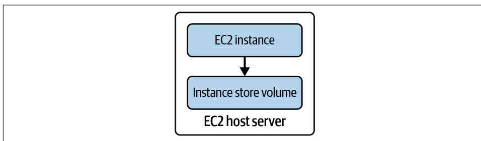
Figure 6-6. Instance store volumes offer high performance and low cost but do not protect data in the event of disk failure or VM shutdown
