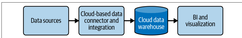
Figure 3-13. Basic components of the modern data stack
