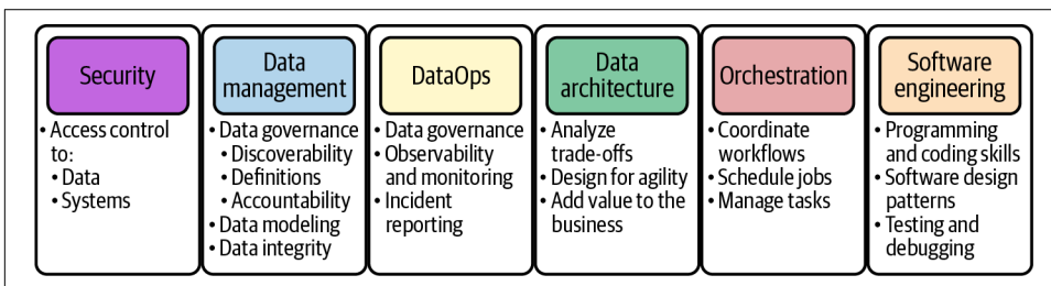
Figure 2-7. The major undercurrents of data engineering
